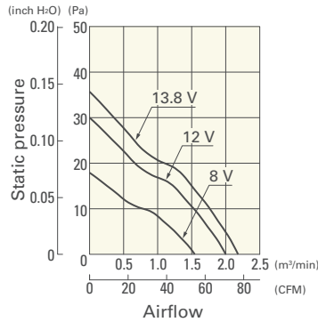
9S1212F401 With pulse sensor
