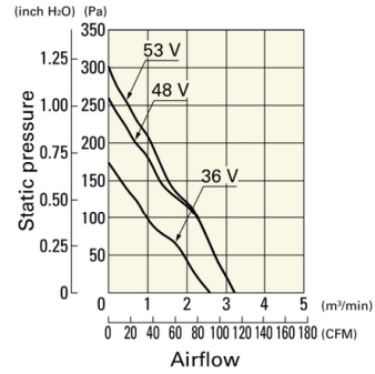
9GA1248S4001 With pulse sensor
