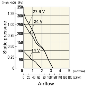
9GA1224S4001 With pulse sensor
