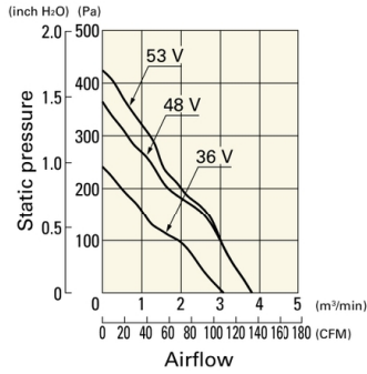
9GA1248G4001 With pulse sensor
